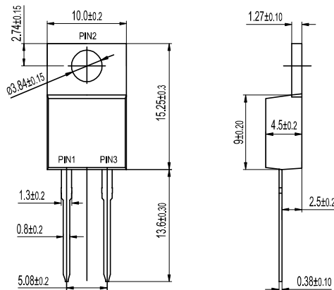
TO-220AC DR20XX
